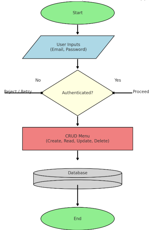
Computer Science Flowchart for Subscription-Based CRUD App in FlutterFlow
